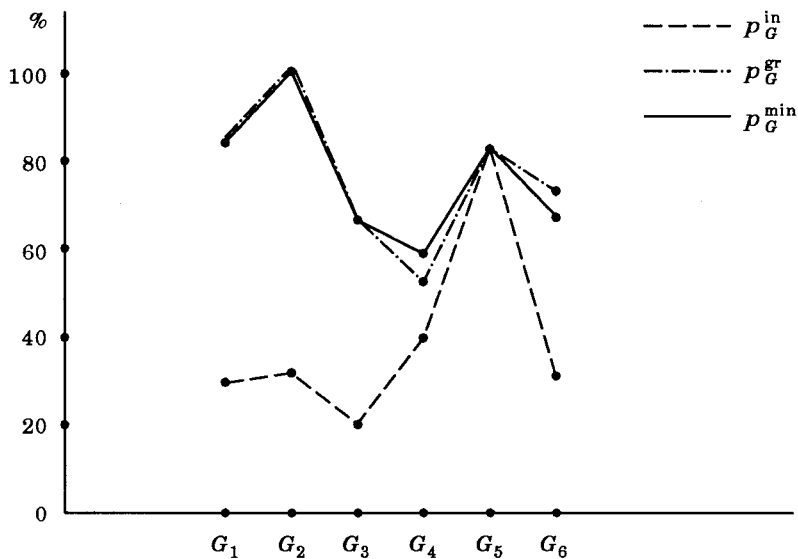
Figure 118. Another proof that the systematic error determined by our calculations is common for all constellations in Zod A. The graph of the percentages of the stars
