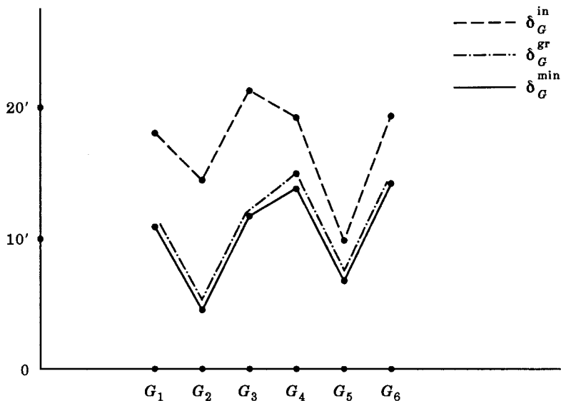
Figure 117. The proof that the systematic error determined by our calculations is common for all constellations in Zod A
